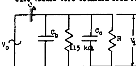
Antenna Equivalent Circuit Boulder, Colorado
